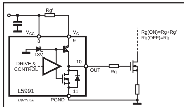
Figure 26. Turn-on and turn-off speeds adjustment.
