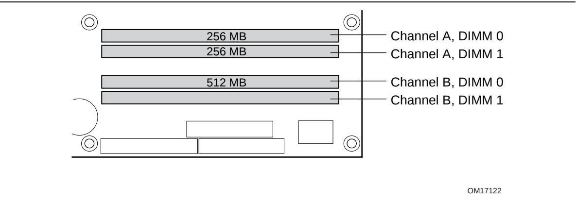
Figure 5. Dual Channel (Interleaved) Mode Configuration with Three DIMMs
