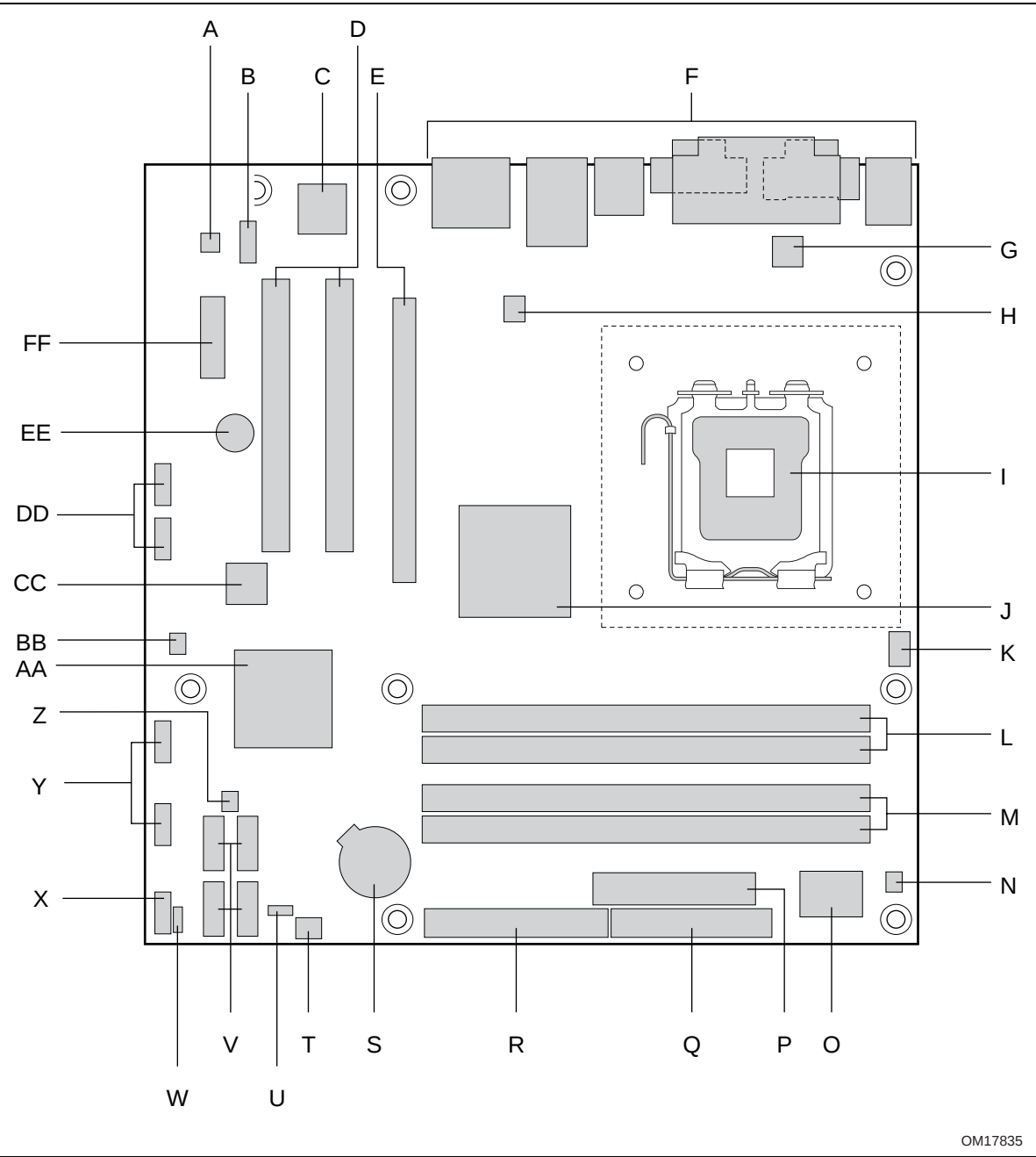
Figure 1. Board Components
