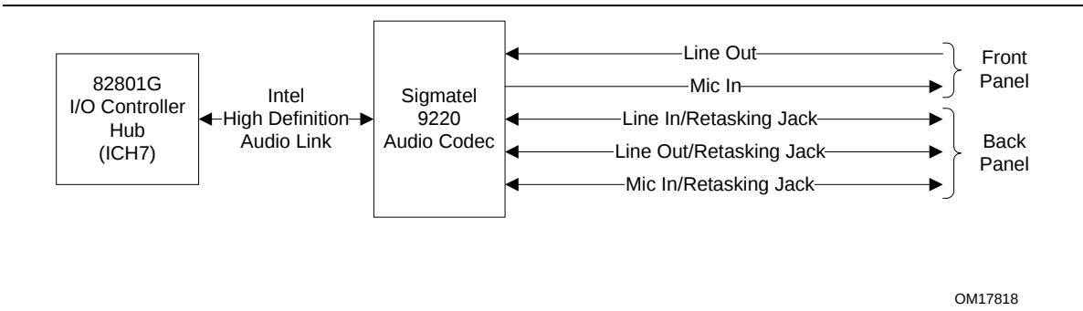
Figure 12. 6-Channel (5.1) Audio Subsystem Block Diagram
