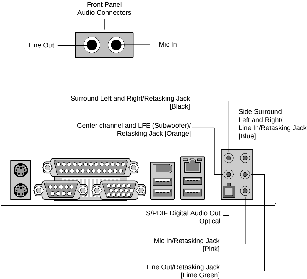
Figure 9. Front/Back Panel Audio Connector Options for 8-Channel (7.1) Audio Subsystem Figure 10 is a block diagram of the 8-channel (7.1) audio subsystem.
