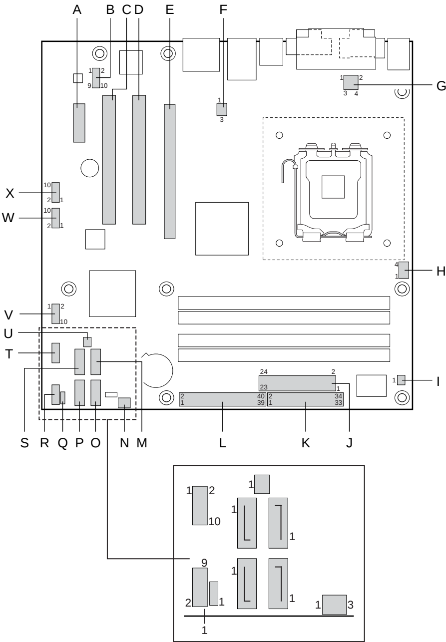
Figure 20. Component-side Connectors
