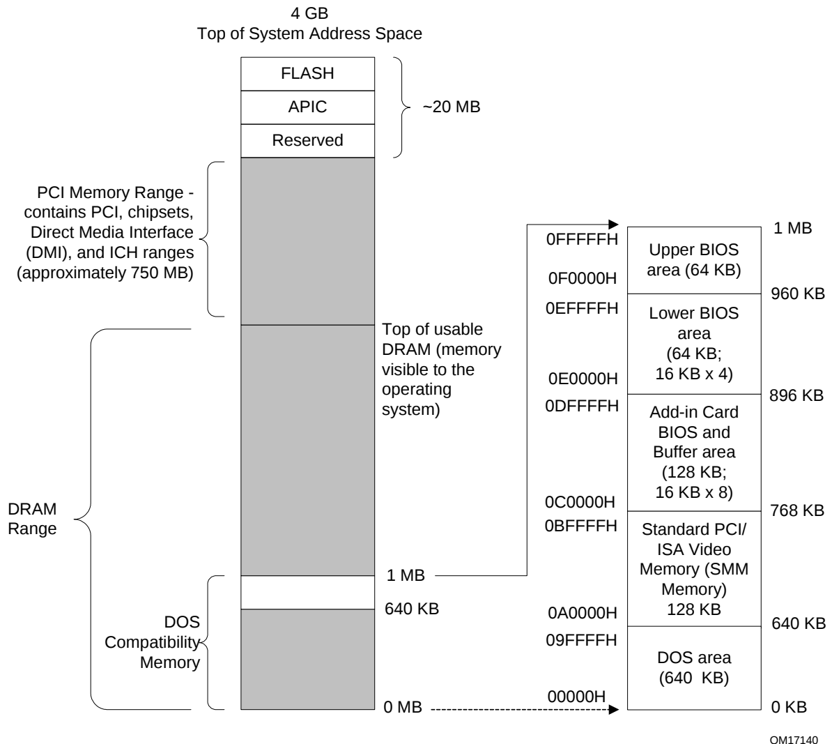
Figure 17. Detailed System Memory Address Map
