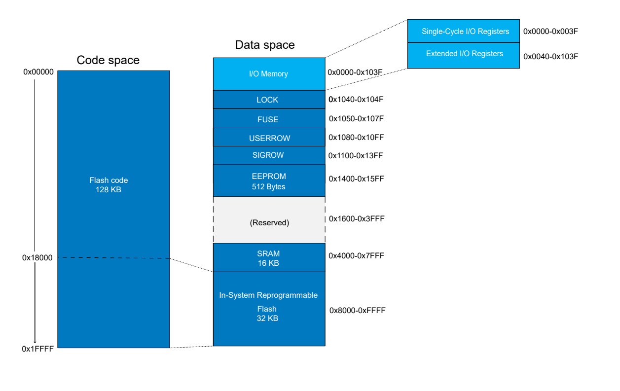
Figure 7-1. Memory Map
