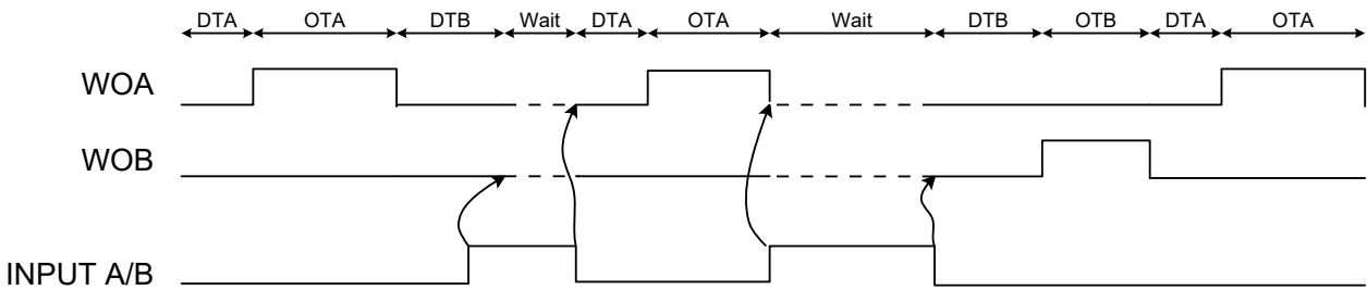
Figure 23-19. Input Mode 6
