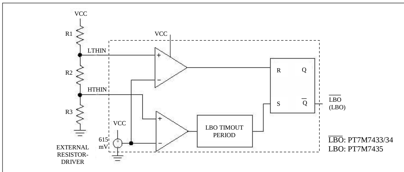
PT7M7433/34/35 Block Diagram
