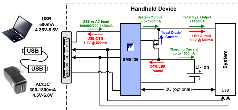
Figure 1 – Using the SMB136 to charge a single cell Li+ battery from USB or AC Adapter power sources
