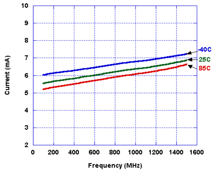
Figure 5. Device Current
