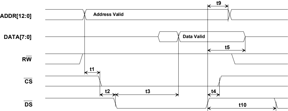
Figure 11-11 Motorola Bus Read Timing (HWMODE = 0, MODEC = 01)
