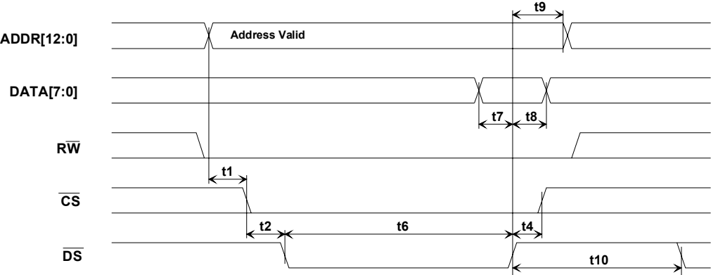
Figure 11-12 Motorola Bus Write Timing (HWMODE = 0, MODEC = 01)
