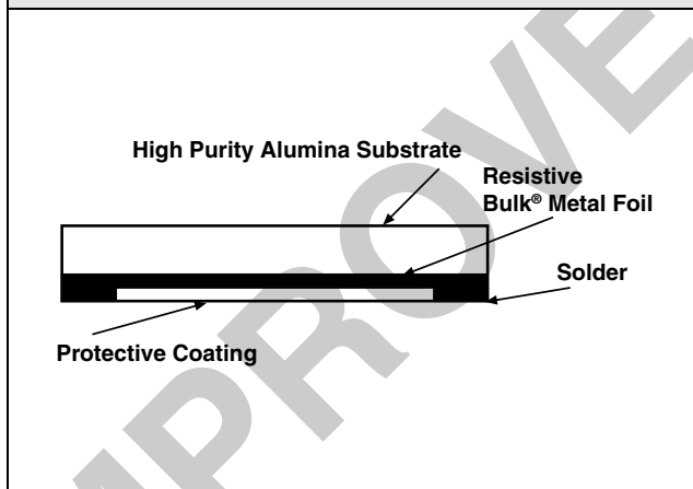
FIGURE 3 - CHIP CONFIGURATION
