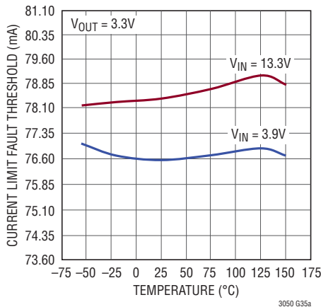
External Current Limit R_{I\text{MAX}} = 1.5k
