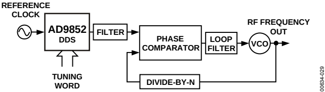
Figure 29. Agile High Frequency Synthesizer
