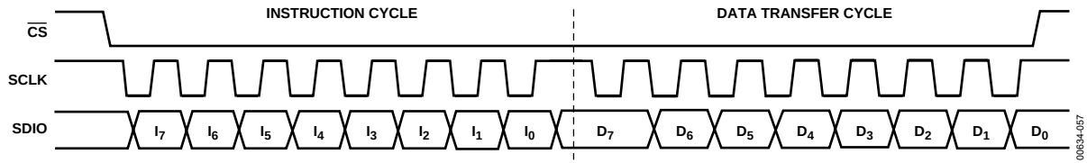
Figure 57. Serial Port Write Timing Clock Stall High
