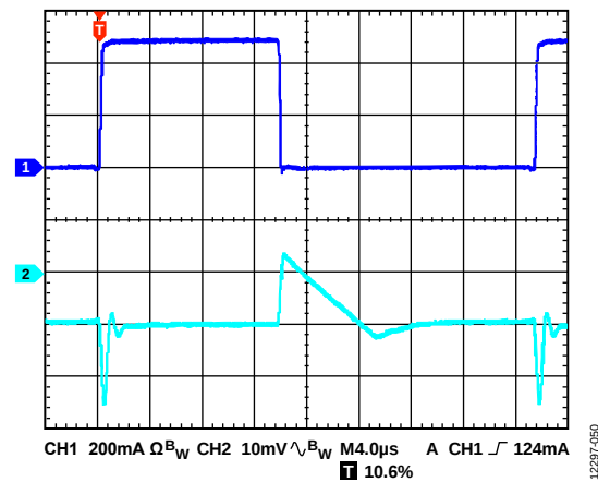
Figure 50. Load Transient Response, I_{LOAD} = 10mA to 510mA , Adjustable Version, V_{OUT} = 1.2V , V_{IN} = 2.5V , CH1 = I_{LOAD} , CH2 = V_{OUT}
