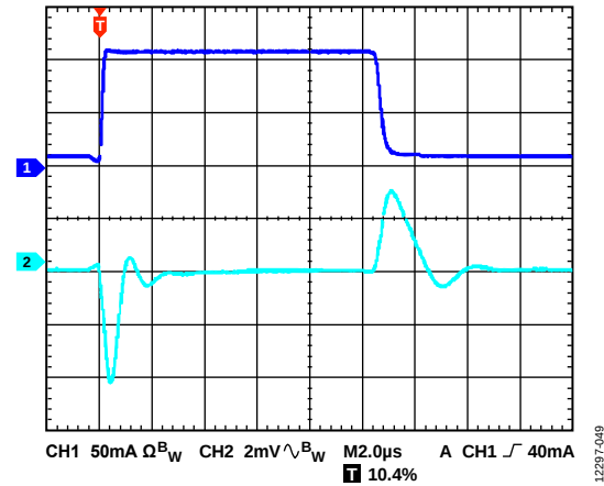
Figure 49. Load Transient Response, I_{LOAD} = 10mA to 110mA , V_{OUT} = 5V , V_{IN} = 5.5V , CH1 = I_{LOAD} , CH2 = V_{OUT}
