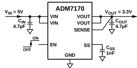
Figure 1. ADM7170 with Fixed Output Voltage, 3.3 V
