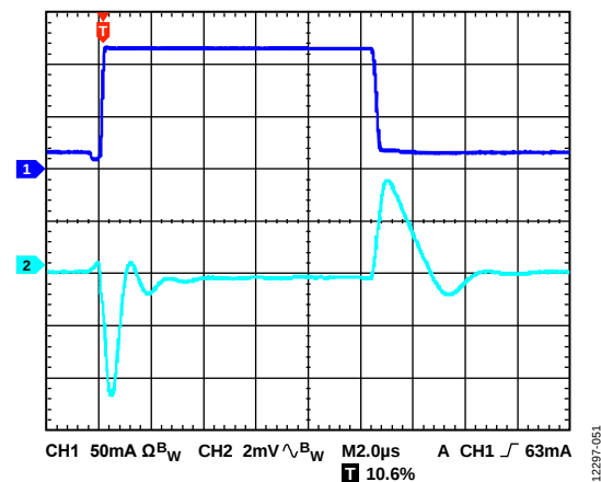
Figure 51. Load Transient Response, I_{LOAD} = 10mA to 110mA , Adjustable Version, V_{OUT} = 1.2V , V_{IN} = 2.5V , CH1 = I_{LOAD} , CH2 = V_{OUT}
