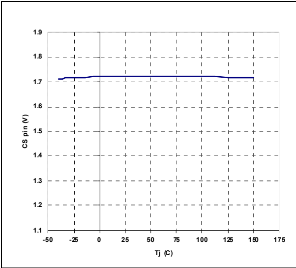
Figure 11. Inductor saturation threshold vs. T_J
