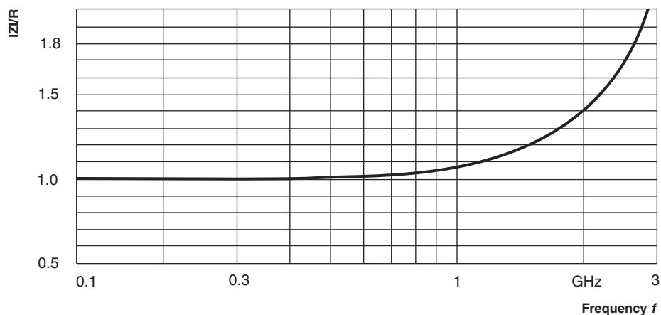
RF - Behaviour
