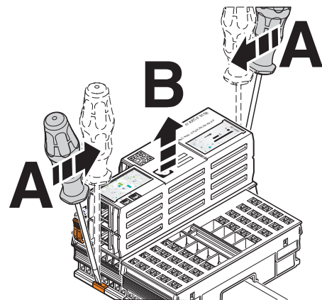
Figure 4 Removing the electronics module
