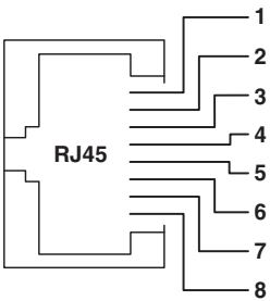
Figure 11 Pin assignment of the Ethernet socket (RJ45)
