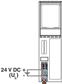
Figure 12 Connection of the cables
