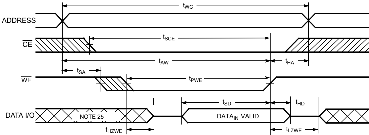
Figure 8. Write Cycle No. 3: \overline{\text{WE}} Controlled, \overline{\text{OE}} LOW [24]
