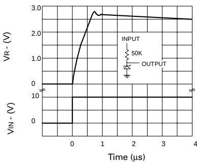
Transient Response ( I_R = 150\mu A )
