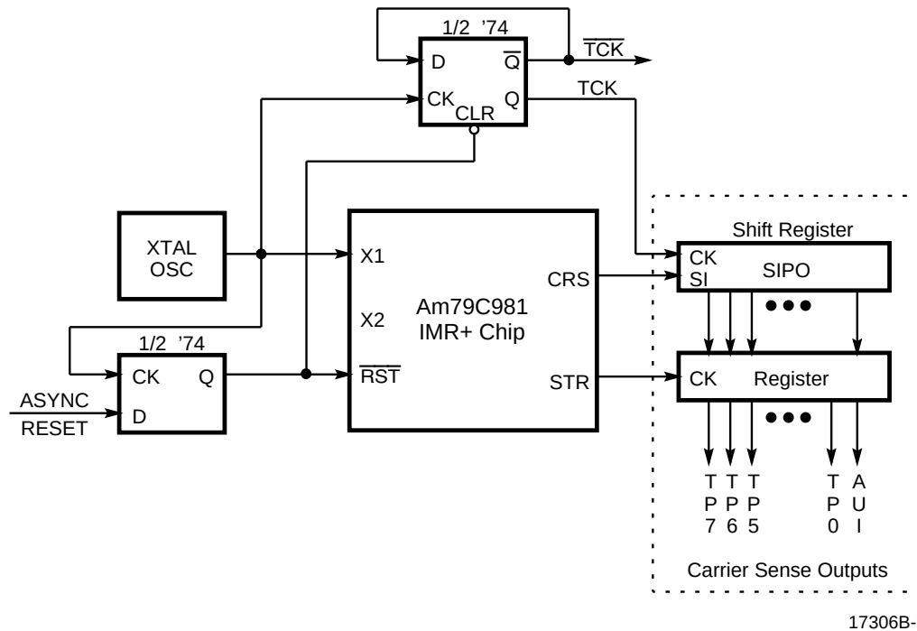
Figure 5a. Port Activity Monitor Implementation
