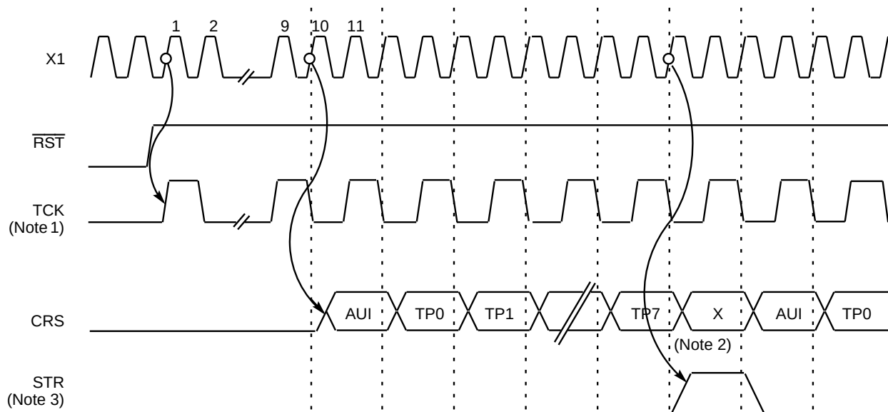
Figure 5a. Port Activity Monitor Implementation
