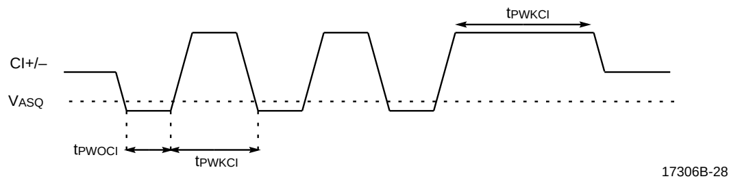
AUI Collision Timing Diagram
