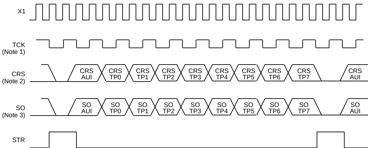
Figure 3. Minimum Mode, Non-Intelligent Repeater Example
