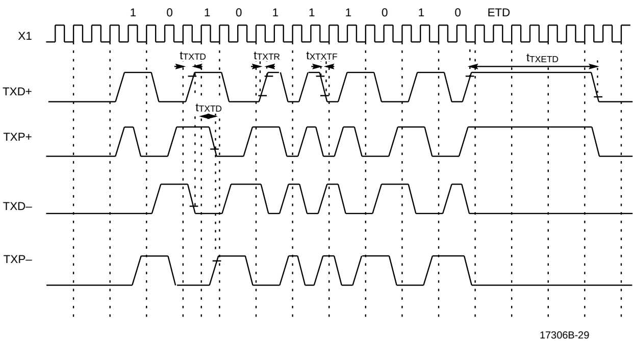
TP Ports Output Timing Diagram
