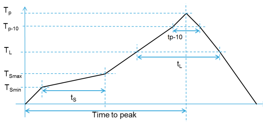
Figure 23. Solder profile
