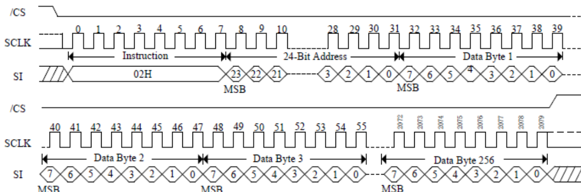
Figure 13. Page Program Sequence Diagram
