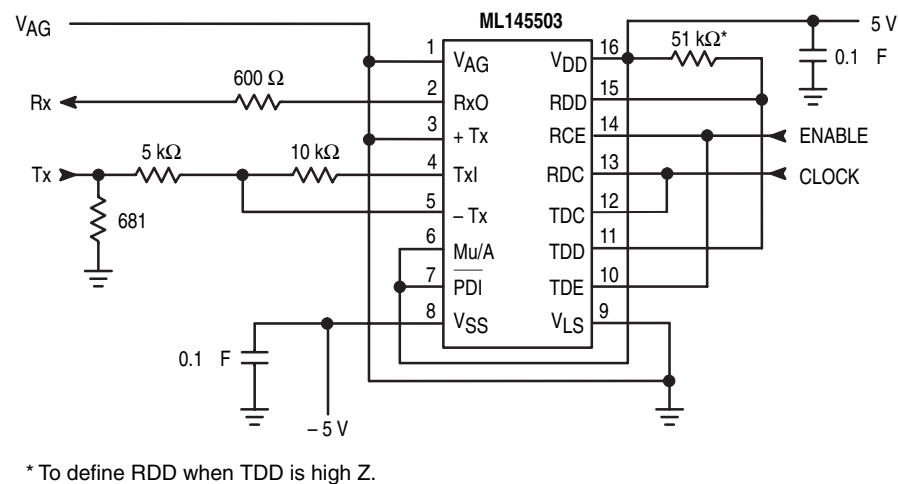
Figure 1. Test Circuit
