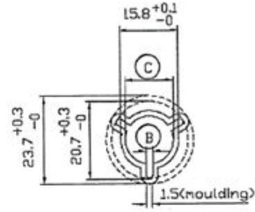
HUB DETAIL
