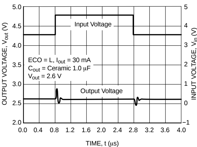
Figure 29. Input Transient Response
