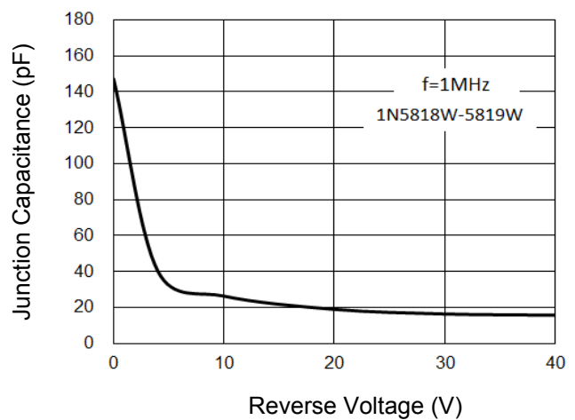
Fig 6. Junction Capacitance
