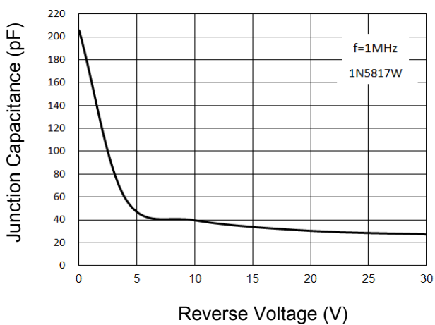
Fig 5. Junction Capacitance
