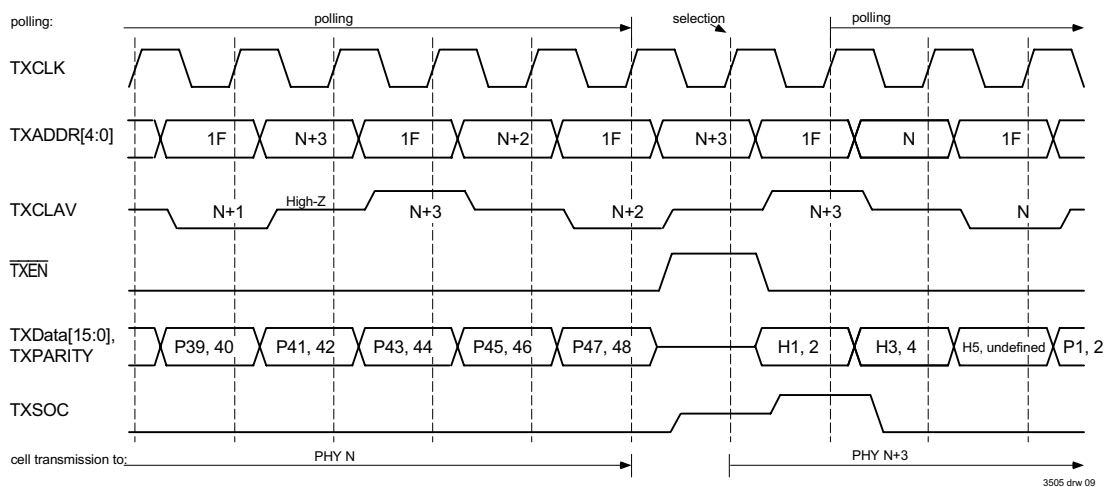
Figure 9 Utopia 2 Transmit Handshake - Back to Back Cells
