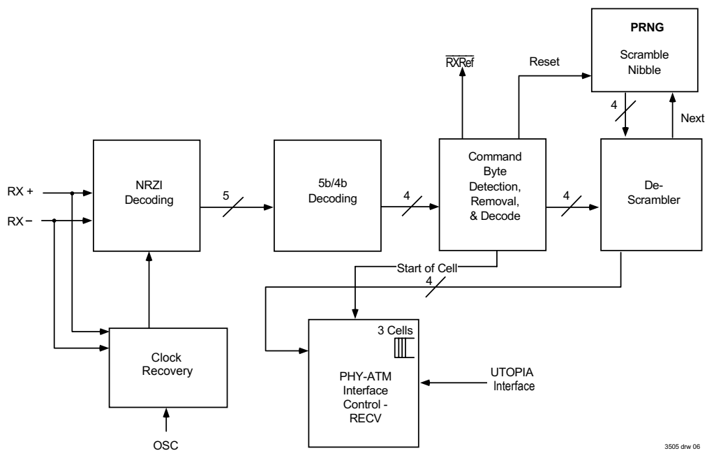
Figure 5 TC Receive Block Diagram
