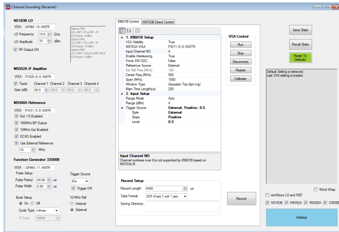
Figure 6. IO control software for RX instrument set up
