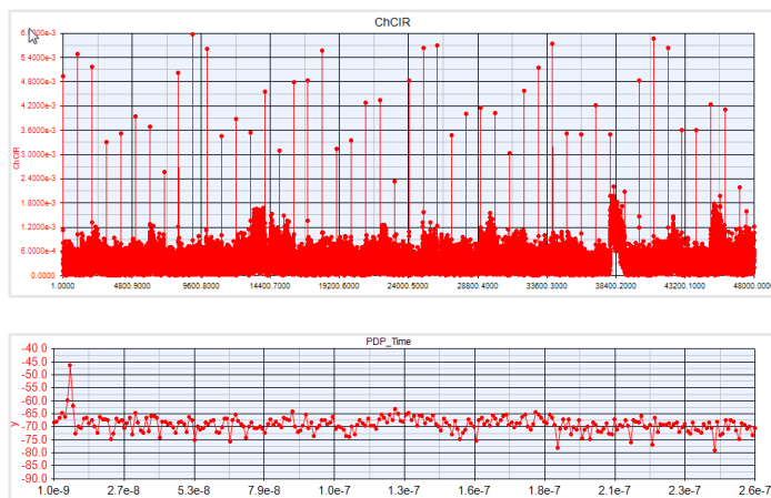
Figure 3. 5G channel sounding CIR results.
