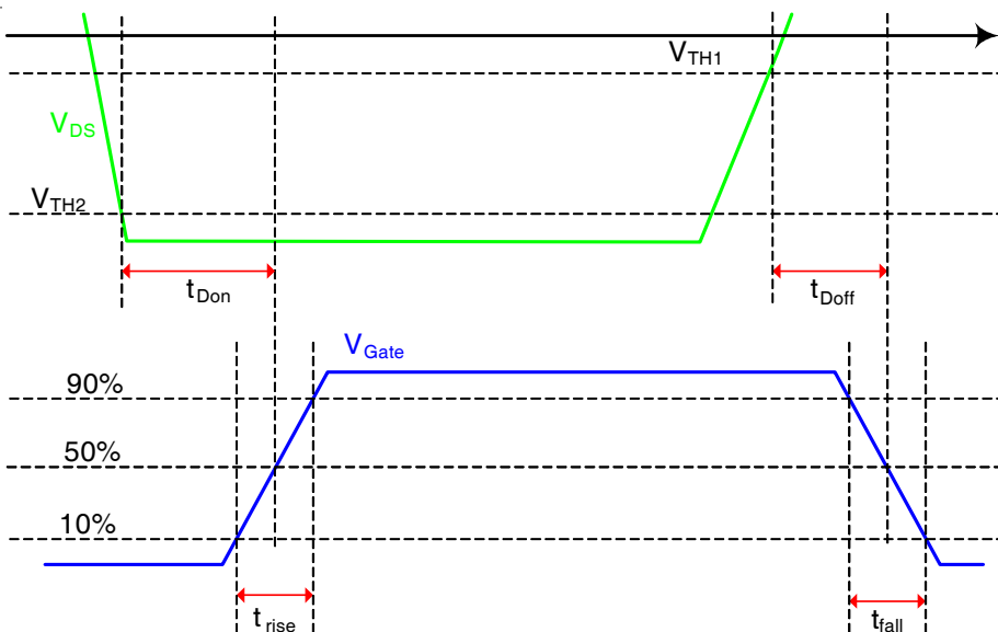
Fig. 15 - Timing Diagrams
