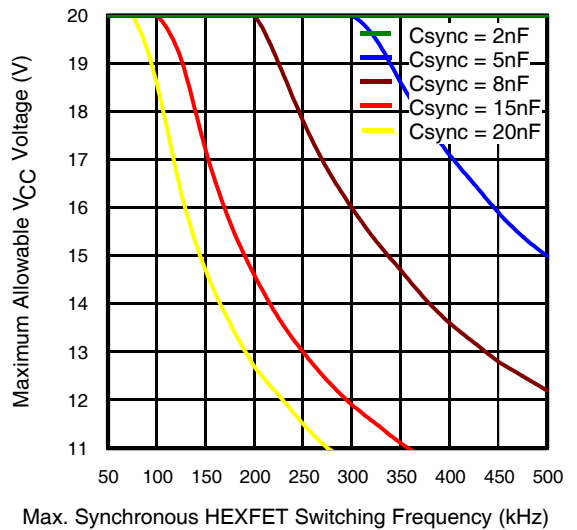
Fig 12. Max. V_{CC} Voltage vs. Synchronous Rectifier Switching Freq, T_J=125^\circ\text{C} , T_{IC} = 85^\circ\text{C} , external R_G=2\Omega , 1\Omega HEXFET Gate Resistance included
