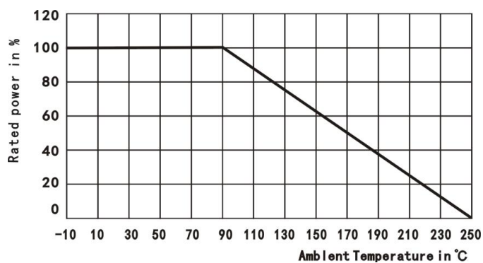
功率曲线 Power Curve
