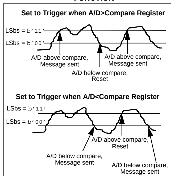
FIGURE 4-1: HYSTERESIS FUNCTION
