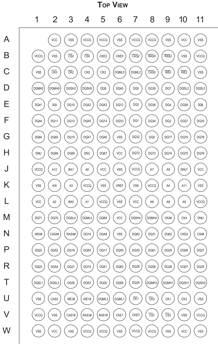
FIG. 1 PIN CONFIGURATION
