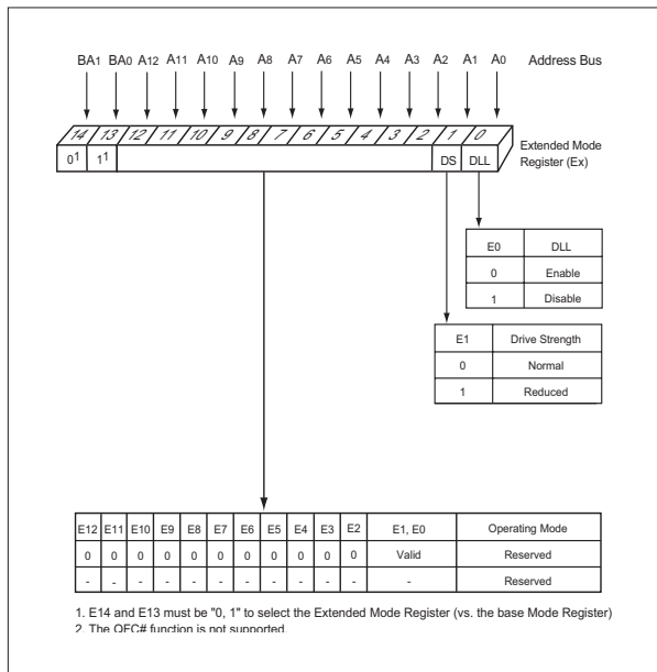
FIG. 5 EXTENDED MODE REGISTER DEFINITION
