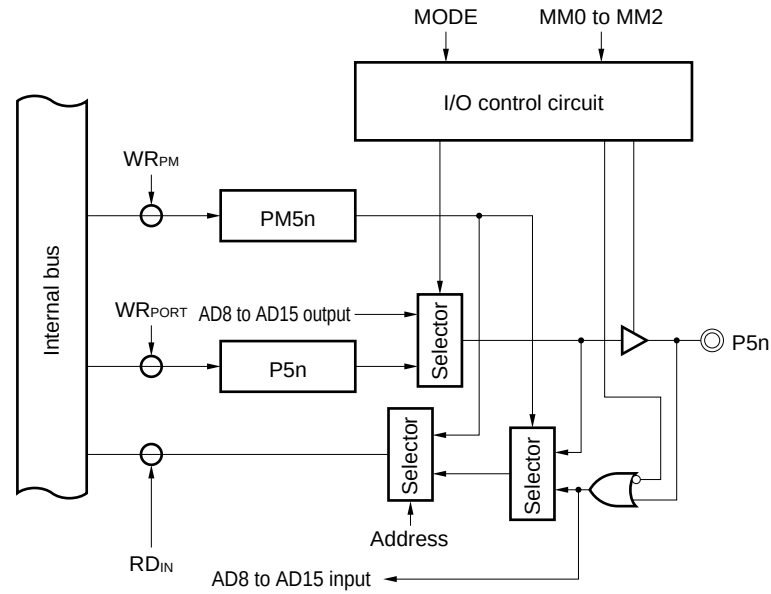
Figure 13-18. Block Diagram of P50 to P57 (Port 5)
