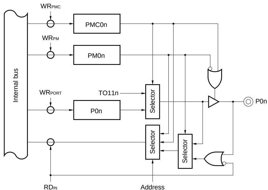
Figure 13-1. Block Diagram of P00 and P01 (Port 0)
