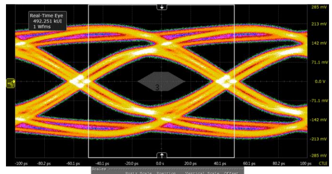
With ESD73004D
