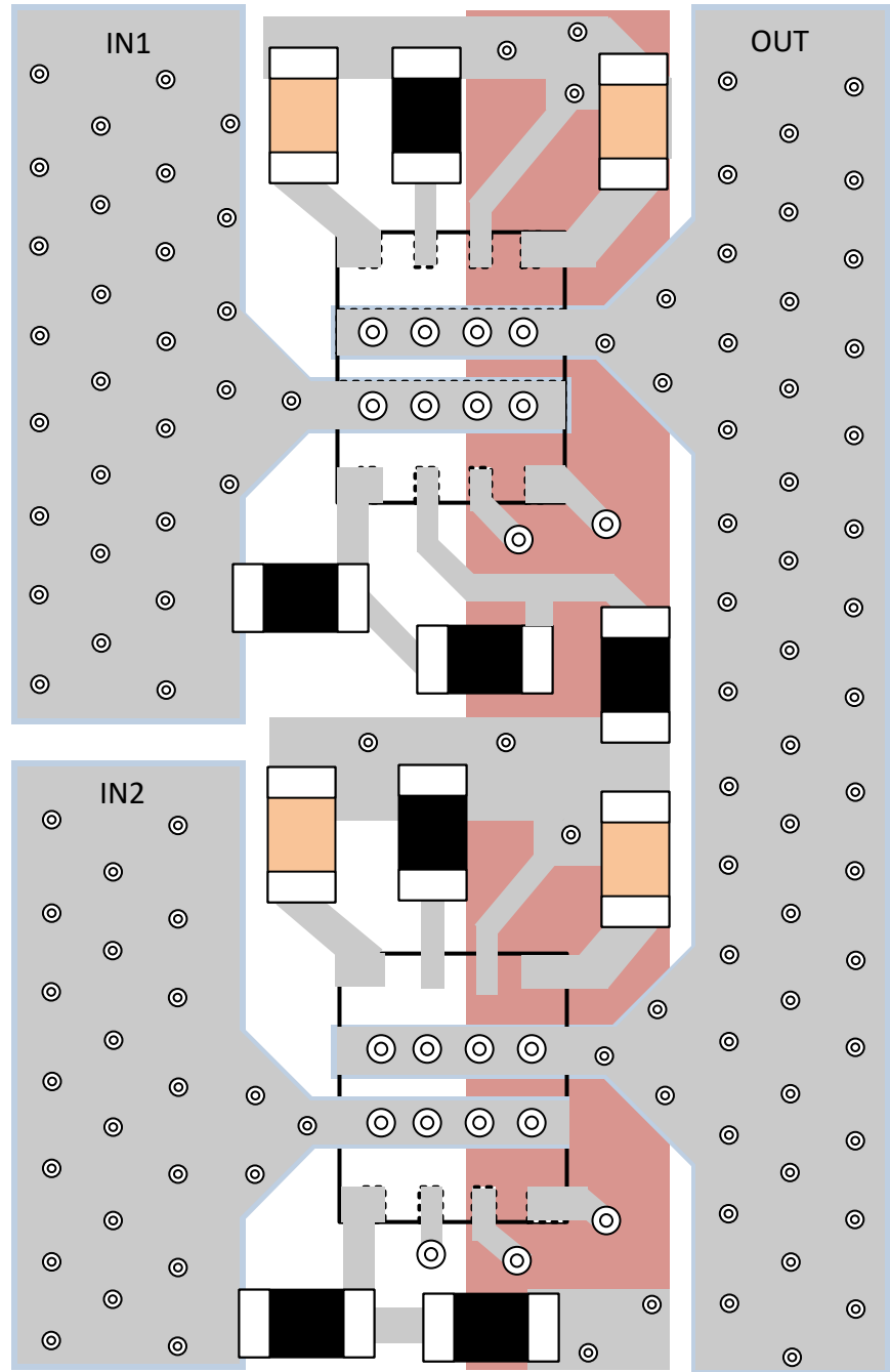
Figure 11-2. Layout Example - 2 x TPS259470x in PowerMUX Configuration
