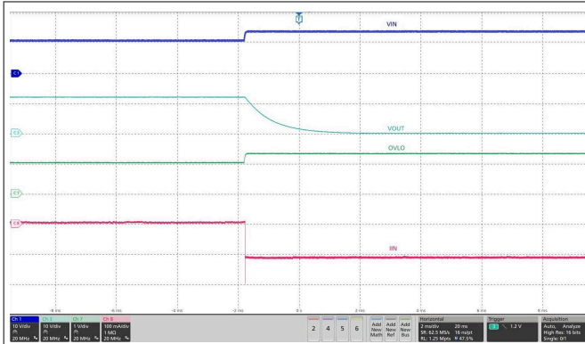
Figure 7-8. Overvoltage Lockout Response - TPS259470x/4x
