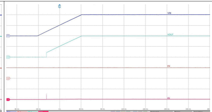
V_{EN/UVLO} = 3.3\text{ V} , C_{OUT} = 22\ \mu\text{F} , C_{dVdt} = \text{Open} , V_{IN} ramped up to 12 V
