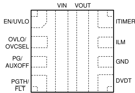
Figure 6-1. TPS25947xx RPW Package 10-Pin QFN Top View
