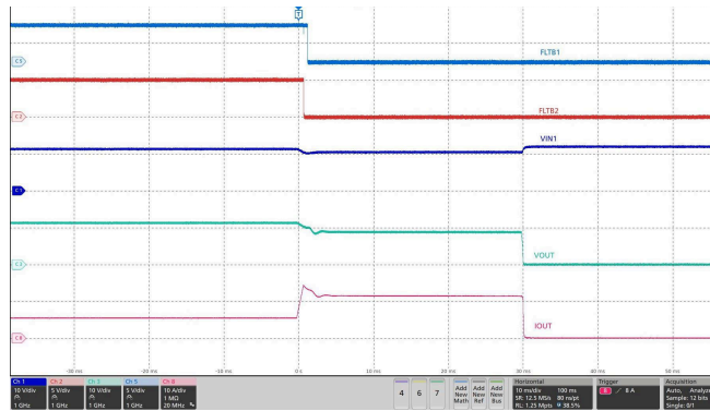
Figure 9-16. Parallel Devices Response to Overload During Steady State
