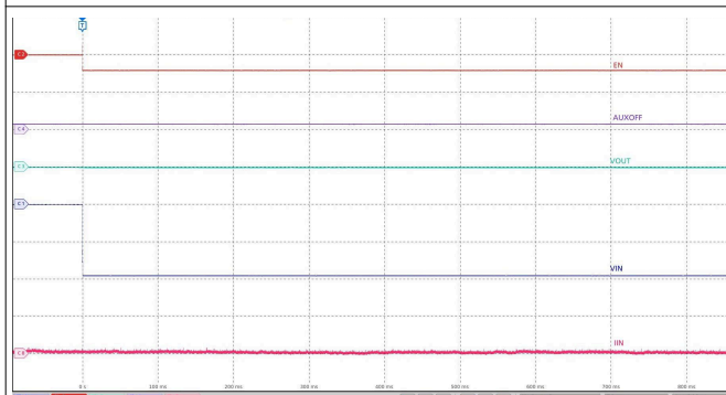
C_{OUT} = 220\ \mu\text{F} , R_{OUT} = 100\ \Omega , V_{IN} stepped down from 0 V to -19 V
