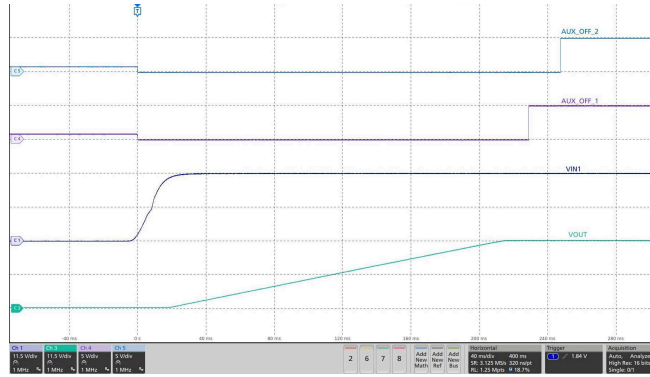
Figure 9-15. Parallel Devices Sequencing During Start-Up
