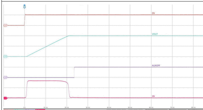
Figure 7-2. Start Up with Enable
