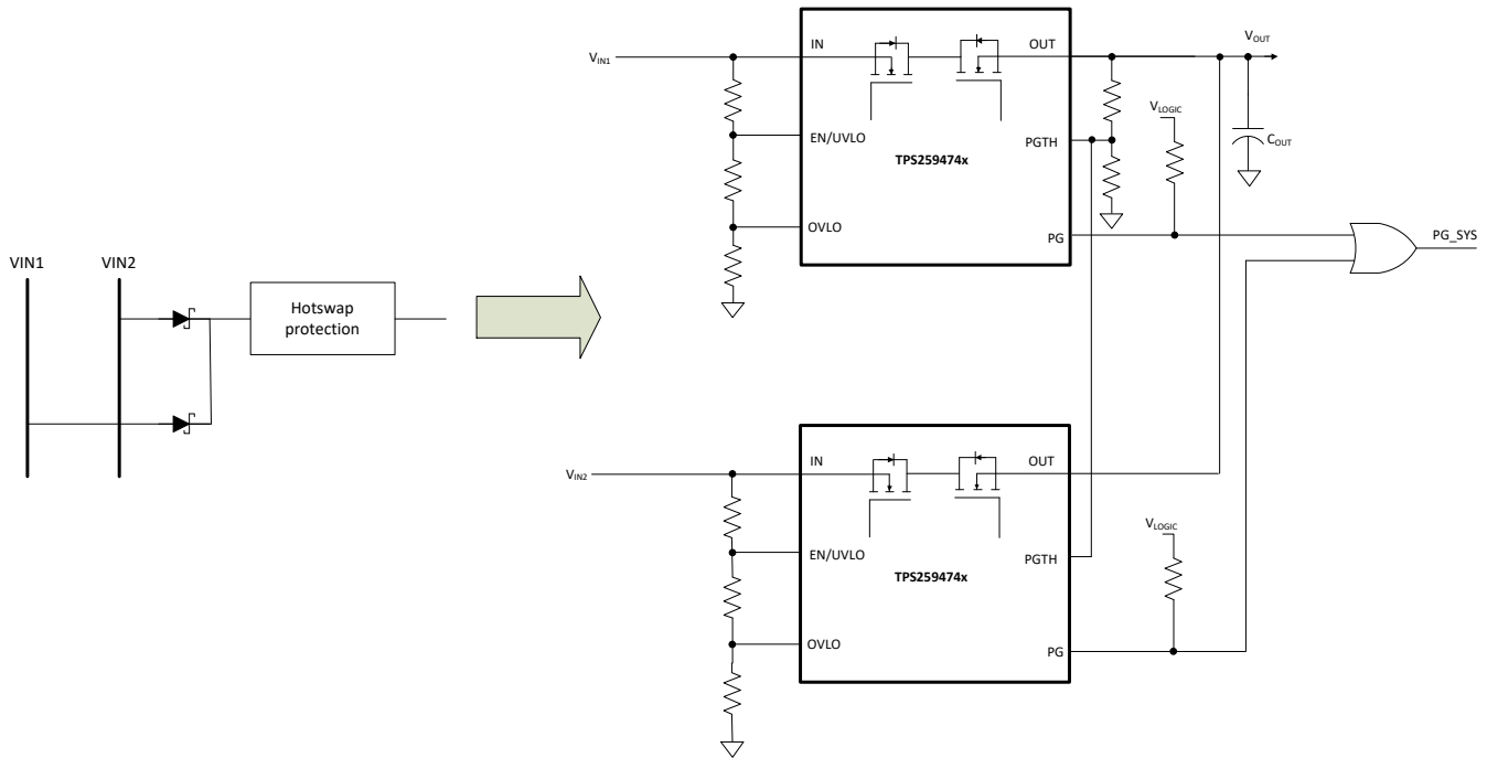
Figure 9-3. Two Devices, Active ORing Configuration
