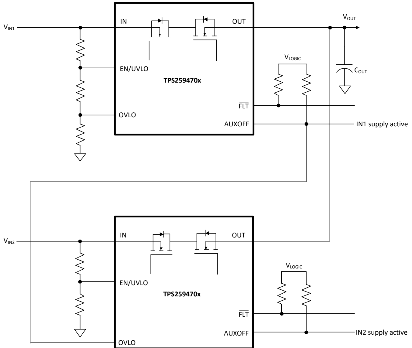
Figure 9-6. Priority Power MUXing with 2 x TPS259470x - Option 1
