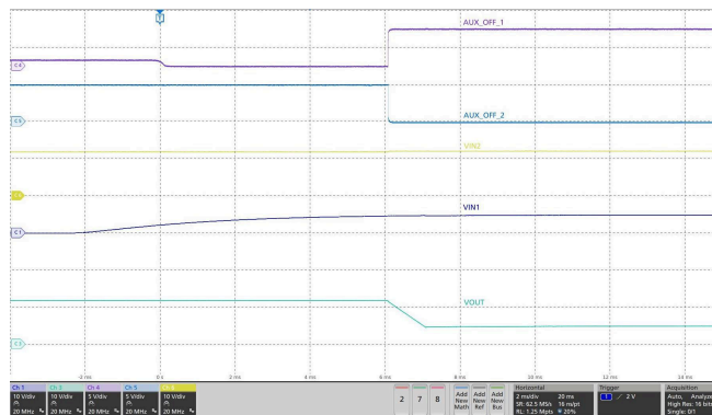
Figure 9-8. TPS259470x Power MUX - Switchover from Auxiliary to Primary Supply
