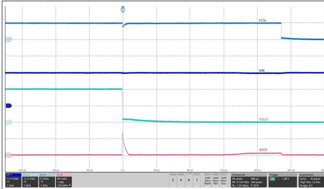
V_{IN} = 12\text{ V} , R_{ILM} = 549\ \Omega , V_{EN/UVLO} = 3.3\text{ V} , OUT stepped from Open \rightarrow Short-circuit to GND
