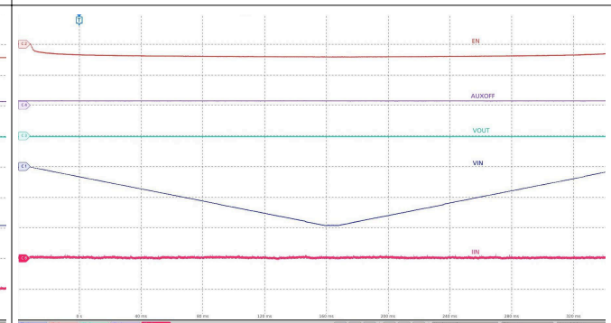
Figure 7-5. Inrush Current with Resistive and Capacitive Load
