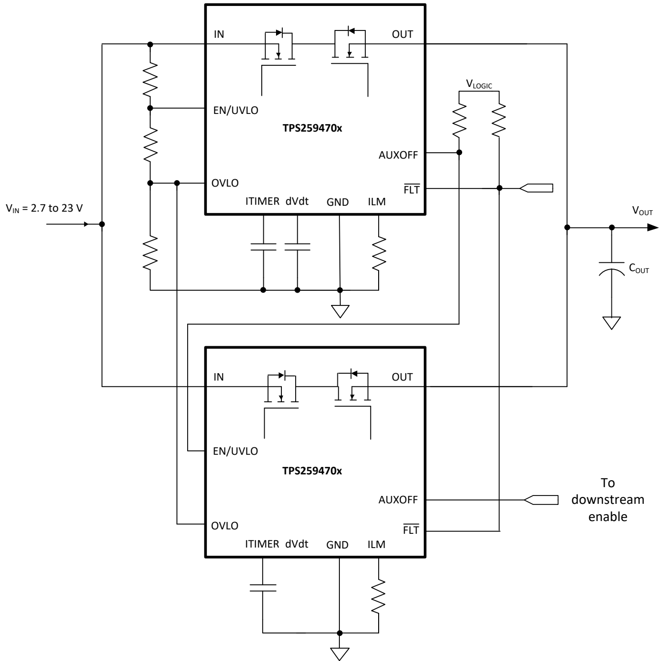
Figure 9-14. Two Devices Connected in Parallel for Higher Steady State Current Capability
