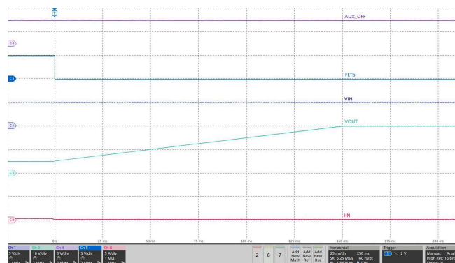
Figure 8-15. Reverse Current Blocking Performance During Slow Voltage Ramp at Output
