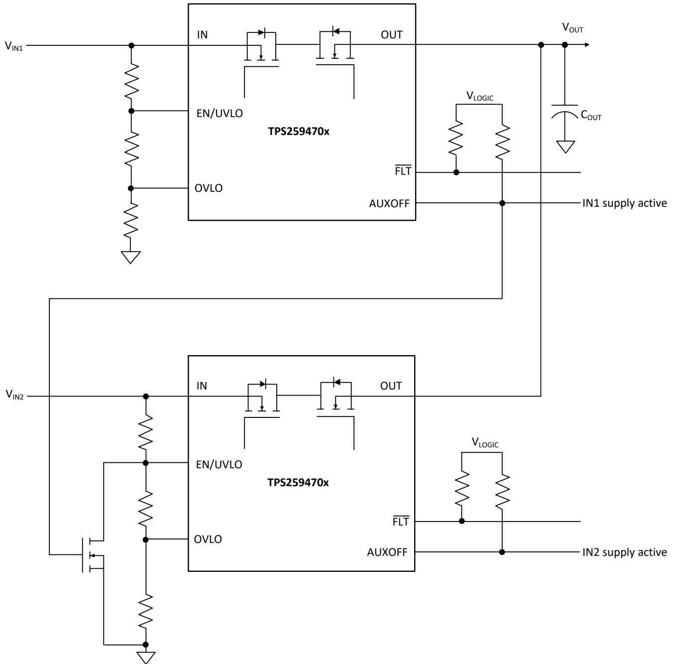
Figure 9-10. Priority Power MUXing with 2 x TPS259470x - Option 3
