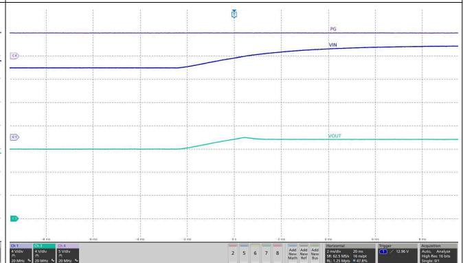
Figure 7-9. Overvoltage Clamp Response - TPS259472x
