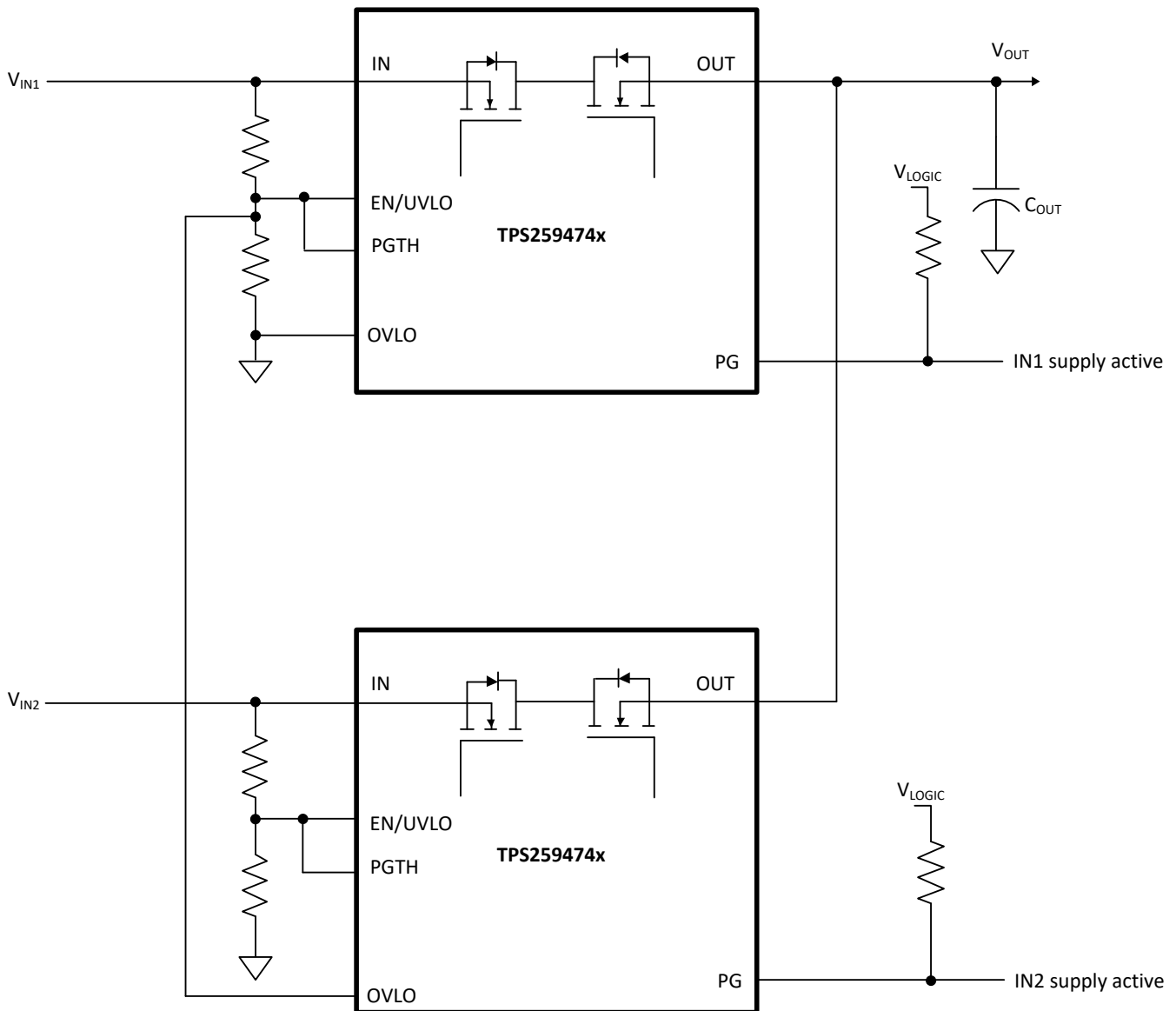
Figure 9-11. Priority power MUXing with 2 x TPS25947x
