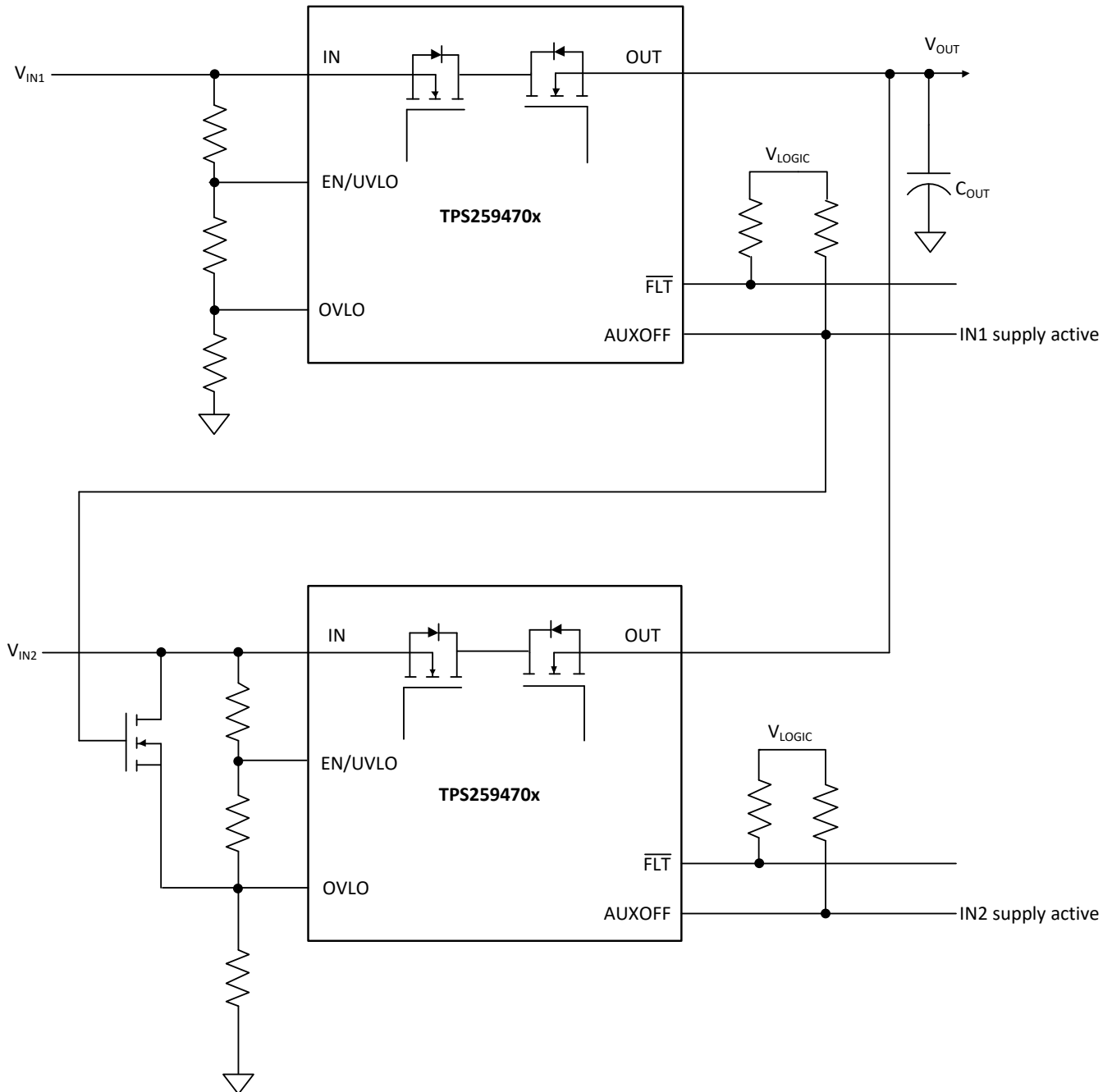
Figure 9-9. Priority Power MUXing with 2 x TPS259470x - Option 2
