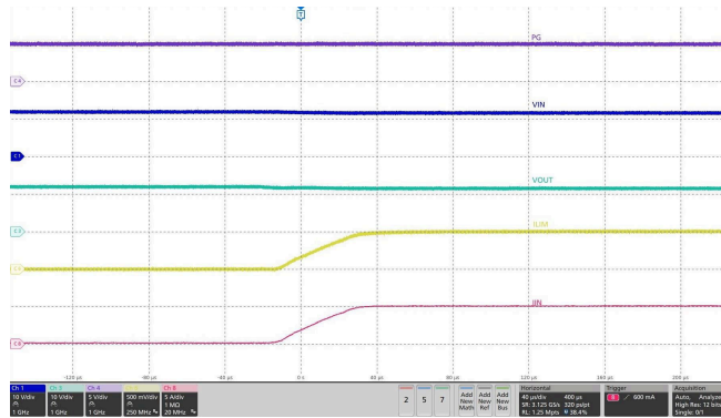
Figure 8-12. Analog Load Current Monitor Response
