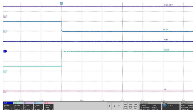
Figure 8-14. Reverse Current Blocking Performance During Fast Voltage Step at Output
