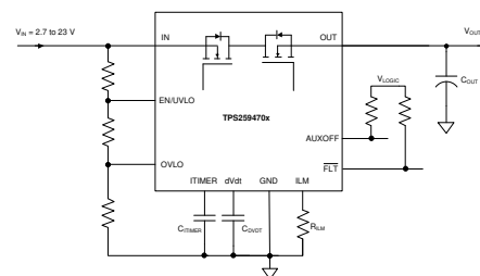
Figure 3-1. Simplified Schematic
