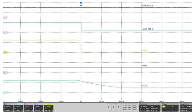
Figure 9-5. Active ORing Response - Supply Ramp Down
