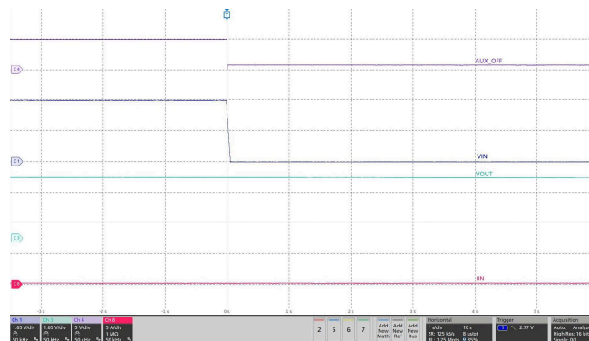
Figure 8-16. Reverse Current Blocking Performance During Input Supply Failure
