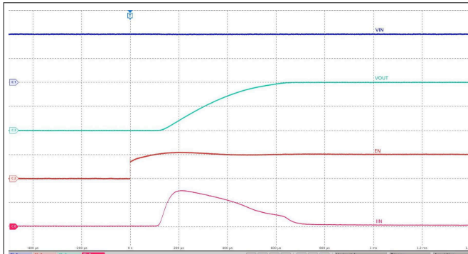
V_{IN} = 12\text{ V} , C_{OUT} = 22\ \mu\text{F} , C_{dVdt} = \text{Open} , V_{EN/UVLO} stepped up to 3.3 V
