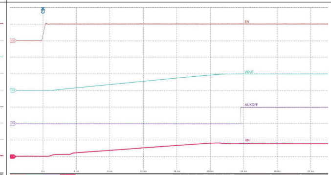
Figure 7-3. Start Up with Supply
