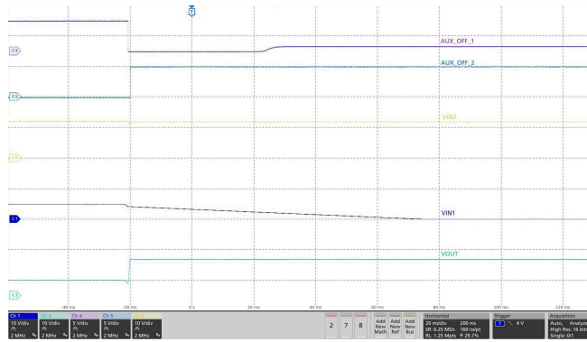
Figure 9-7. TPS259470x Power MUX - Switchover from Primary to Auxiliary Supply
