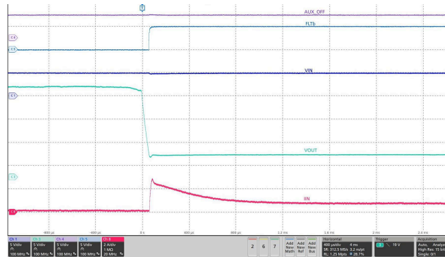
Figure 9-13. TPS259470x 5-V Source Path - USB Fast Role Swap Response
