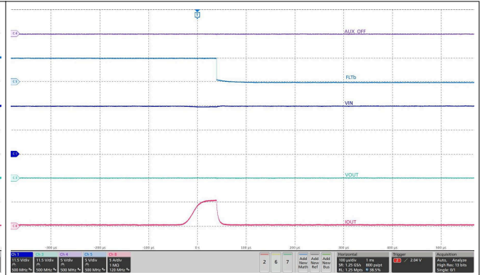
V_{IN} = 23\text{ V} , C_{OUT} = \text{Open} , OUT short-circuit to GND, R_{ILM} = 549\ \Omega , V_{EN/UVLO} stepped from 0 V to 3.3 V
