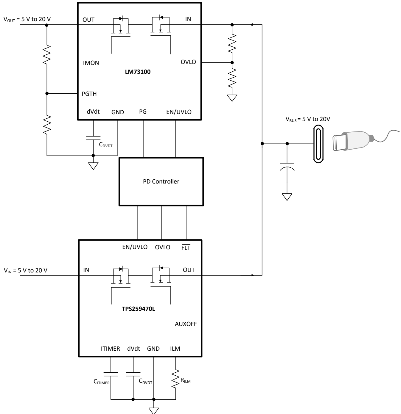
Figure 9-12. USB PD Port Protection
