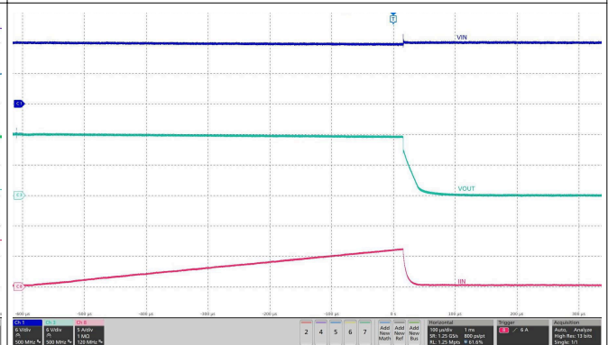
Figure 7-11. Overvoltage Clamp Response - TPS259472x
