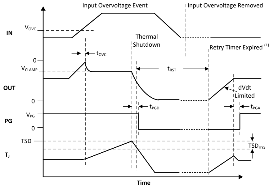
Figure 8-8. TPS259472x Overvoltage Response (Auto-Retry)
