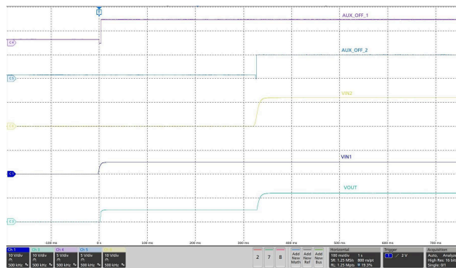
Figure 9-4. Active ORing Response - Supply Ramp Up
