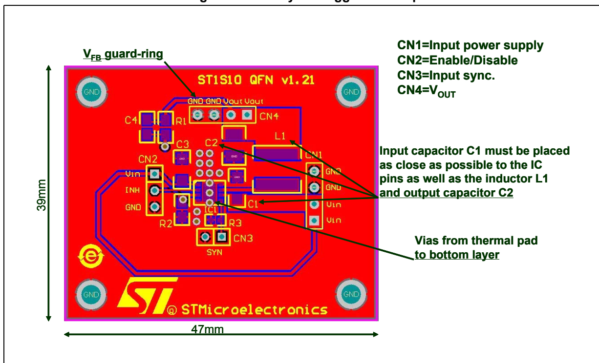
Figure 6. PCB layout suggestion - top
