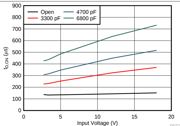
图 22. Turn on Delay vs Input Voltage
