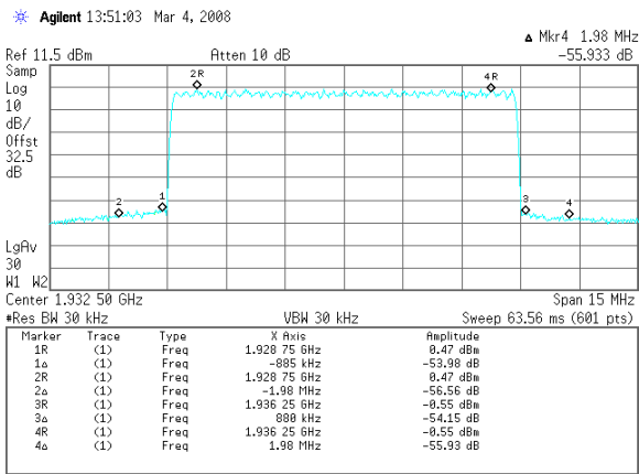
Spurious Emission @ Fc 1932.5MHz, CDMA 7FA, 32dBm
