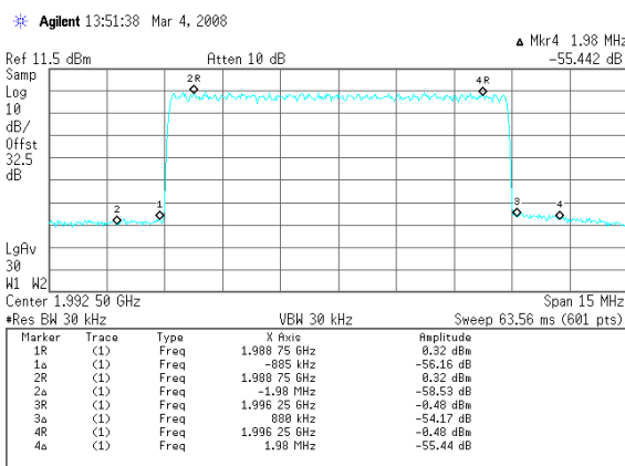
Spurious Emission @ Fc 1992.5MHz, CDMA 7FA, 32dBm
