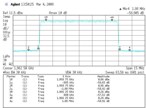
Spurious Emission @ Fc 1962.5MHz, CDMA 7FA, 32dBm
