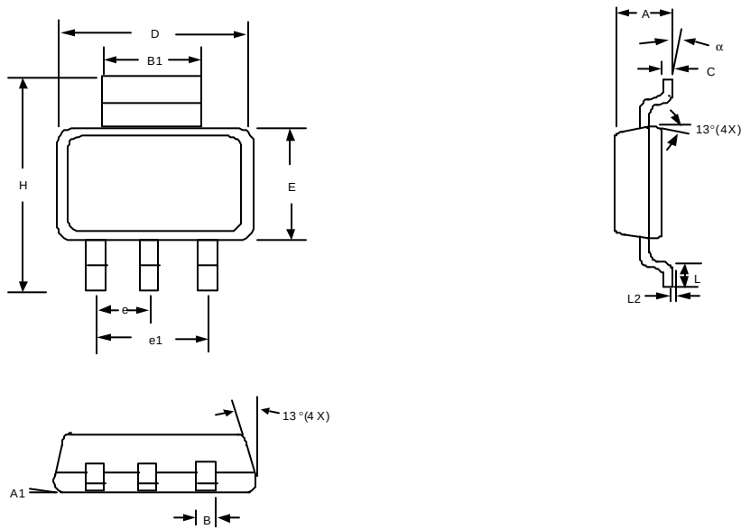
SOT-223 (T6) Package
