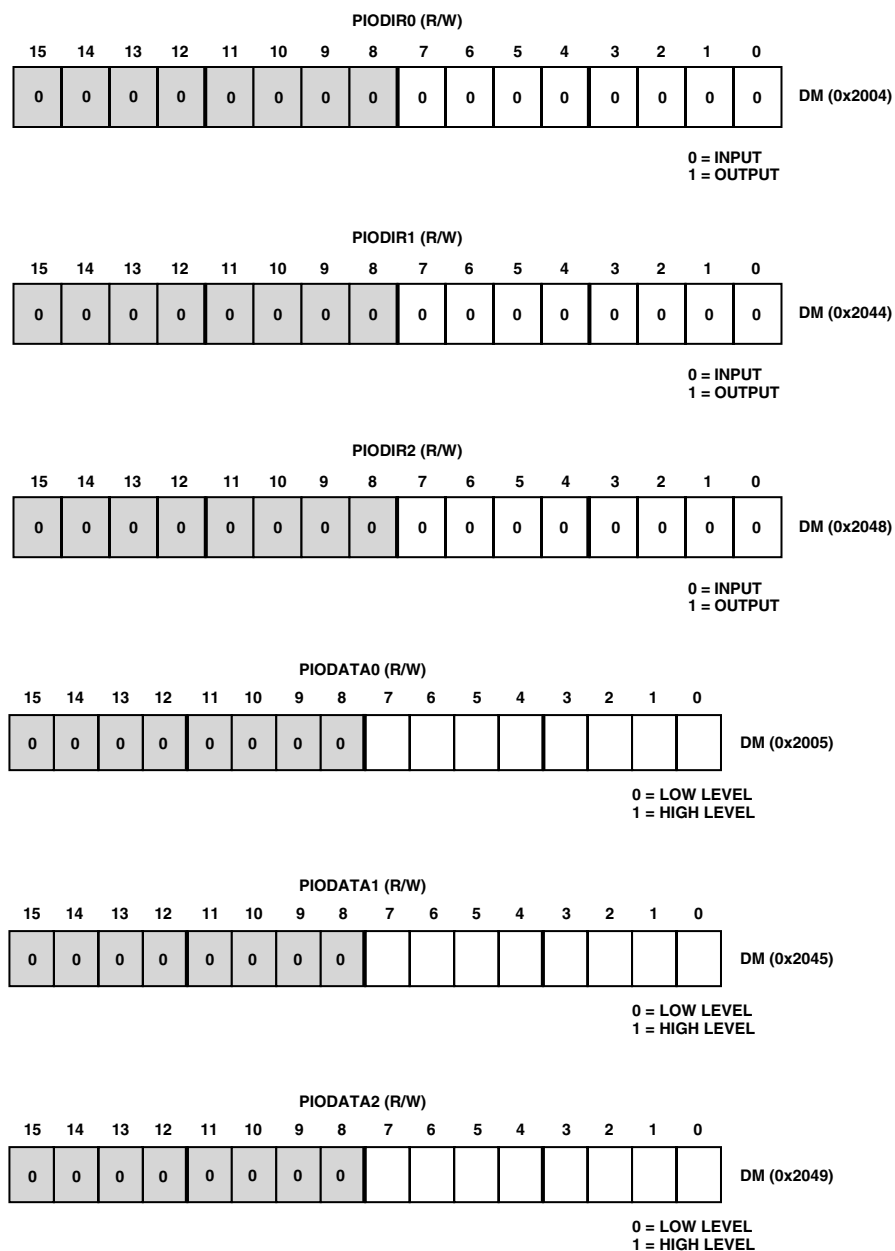
Figure 18. Configuration of ADC331 Registers
