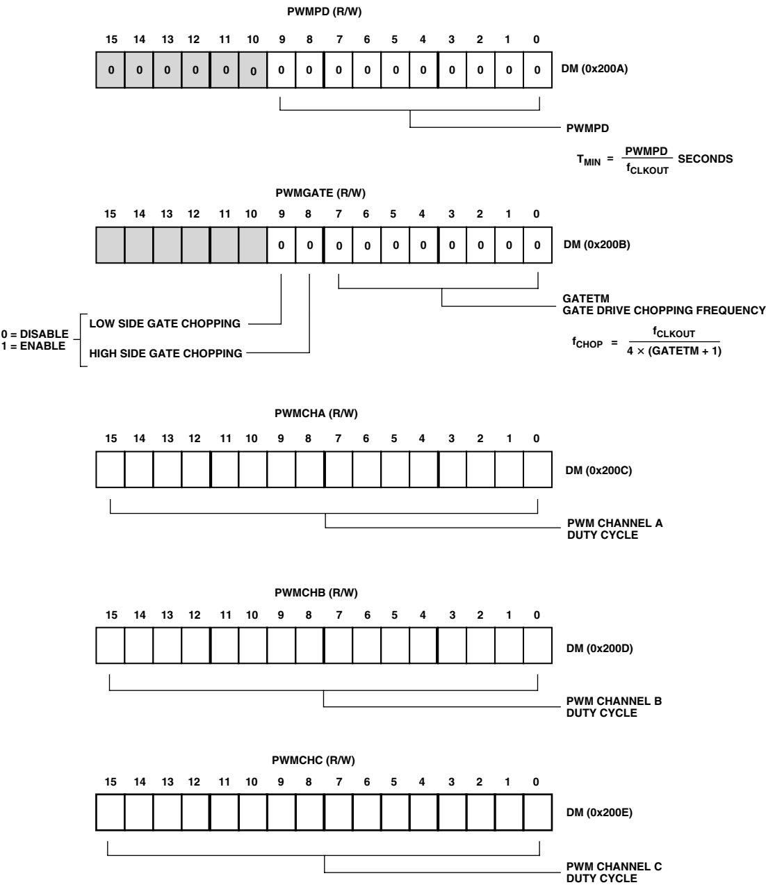
Figure 17. Configuration of ADCM331 Registers
