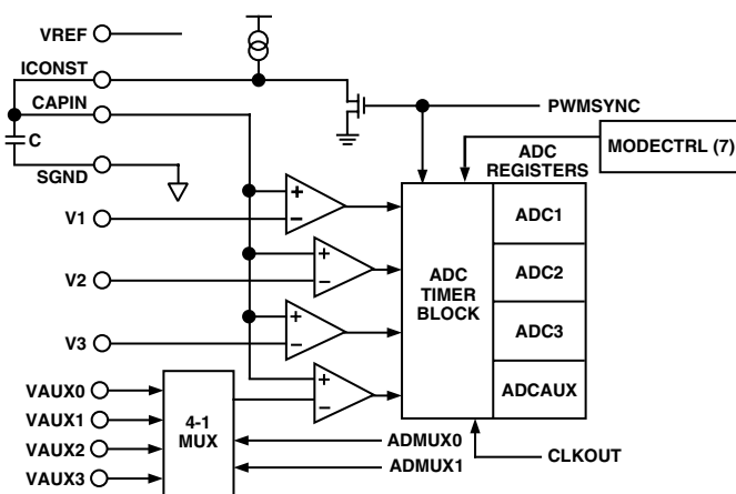
Figure 11. ADC Overview
