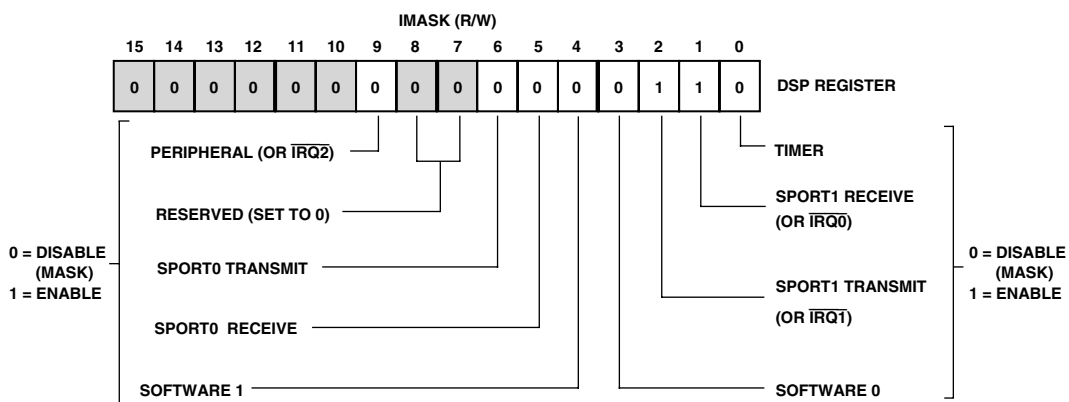
Figure 23. Configuration of ADMC331 Registers
