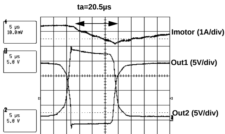
Figure 15. Switch off Time
