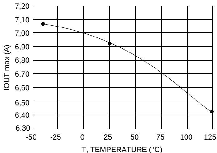
Figure 14. Current Limitation
