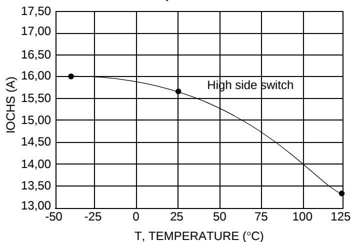
Figure 13. Over Current Detection versus Temperature
