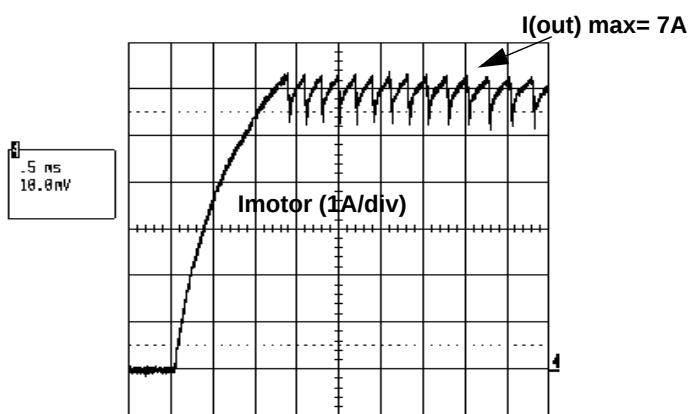
Figure 14. Current Limitation
