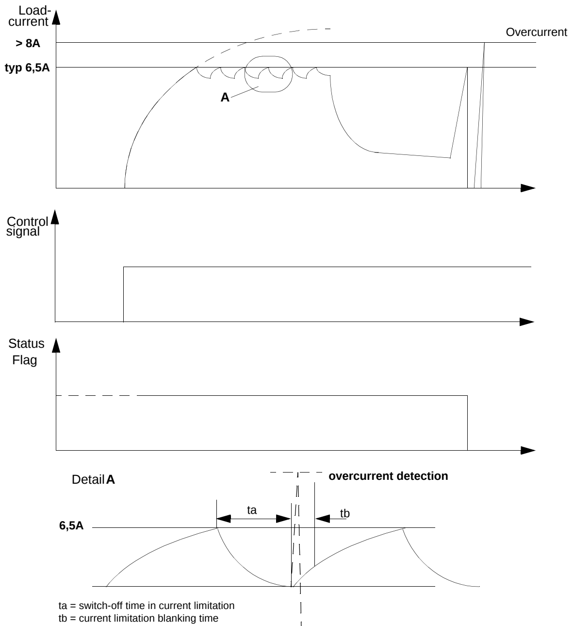
Figure 5. Current Limitation
