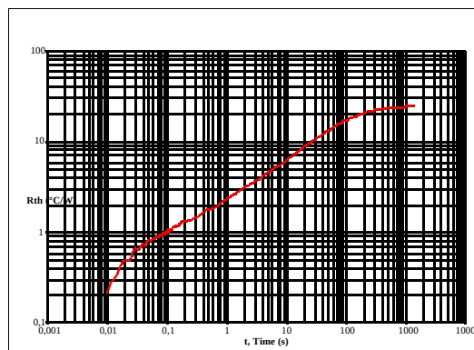
Figure 23. PHSOP20 Thermal Response
