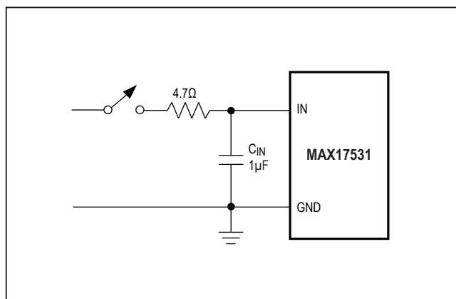
Figure 4. Transient Protection
