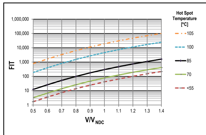
FIT @ Hot Spot Temperatures
