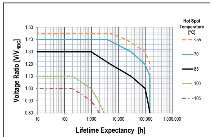
Lifetime Curve V_{NDC} = 900 V- and V_{NDC} = 1,100 V-
