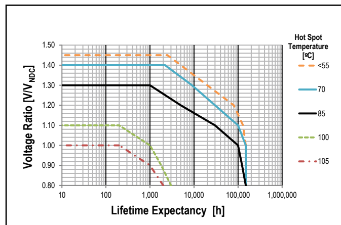
Lifetime Curve V_{NDC} = 600 V- and V_{NDC} = 700 V-
