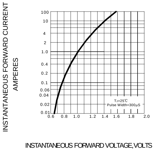
FIG.4-TYPICAL FORWARD CHARACTERISTIC
