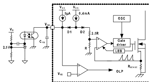
Figure 16. Pulse-Width-Modulation Circuit
