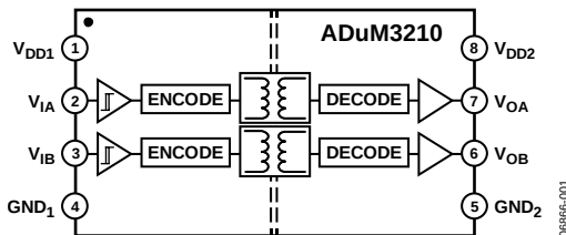
Figure 1. ADuM3210
