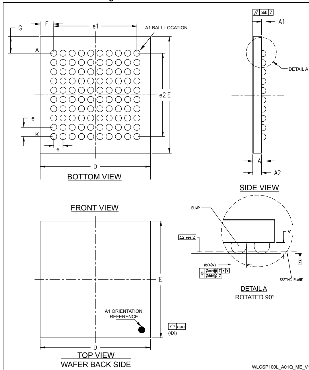
Figure 98. WLCSP100 outline
