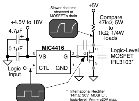
Figure 5. MOSFET Capacitance Effects at High Switching Frequency
