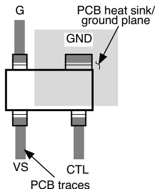
Figure 4. Heat-Sink Plane
