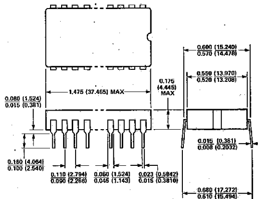
28 LEAD CERDIP (JI)
