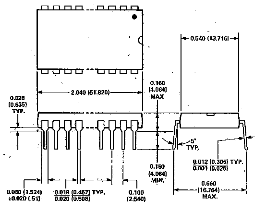
40 LEAD PLASTIC (PL)
