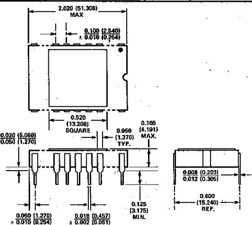
40 LEAD CERAMIC (DL)
