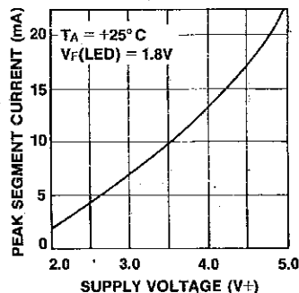
SEGMENT CURRENT VS SUPPLY VOLTAGE
