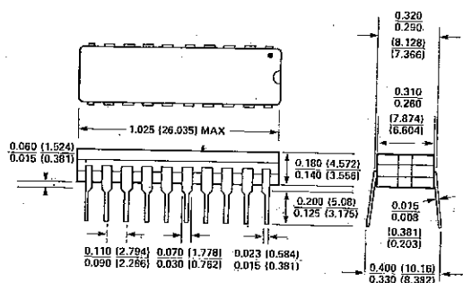
20 LEAD CERDIP (JP)
