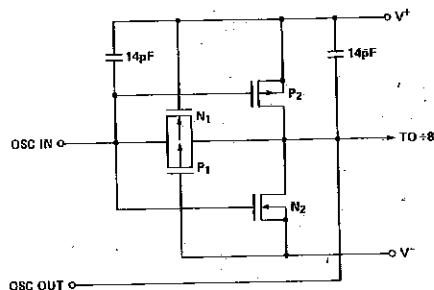
ICM7206 Oscillator
