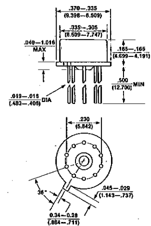
TO-100 (TW, TX)
