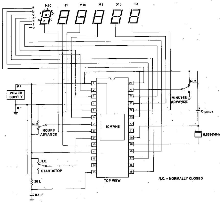
Figure 2: Clock Mode
