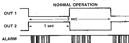
OUTPUT WAVEFORMS (ICM1115)
