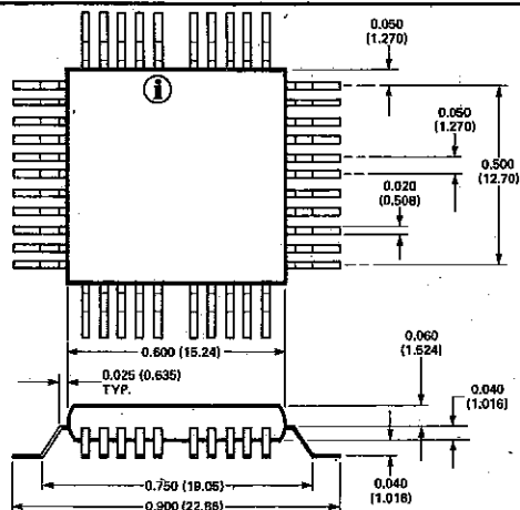
42 PIN FLATPACK (BH)
