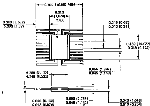
24 LEAD FLATPACK (FG)
