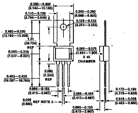
TO-202
