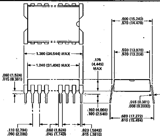
28 LEAD PLASTIC (PI-1)
