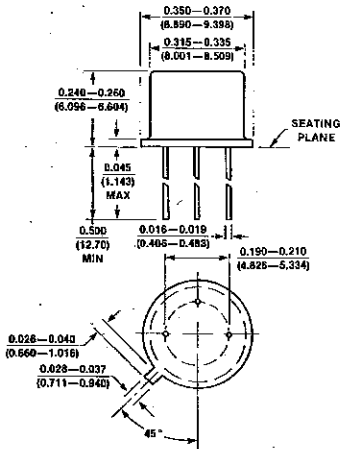
TO-39
