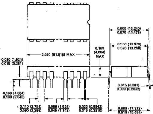
40 LEAD CERDIP (JL)
