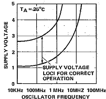
SUPPLY VOLTAGE RANGE FOR CORRECT OPERATION OF \div 8 COUNTER AS A FUNCTION OF OSCILLATOR FREQUENCY
