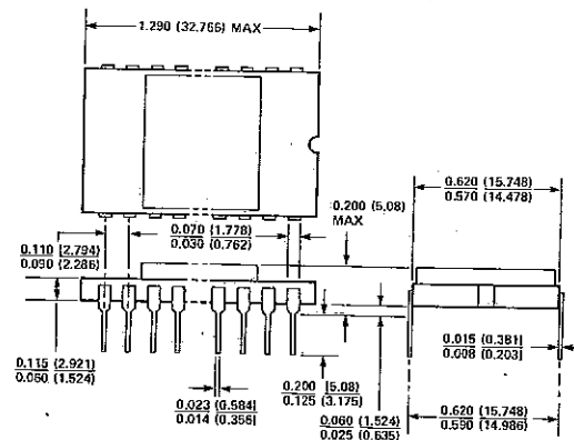
22 LEAD CERDIP (JF)
