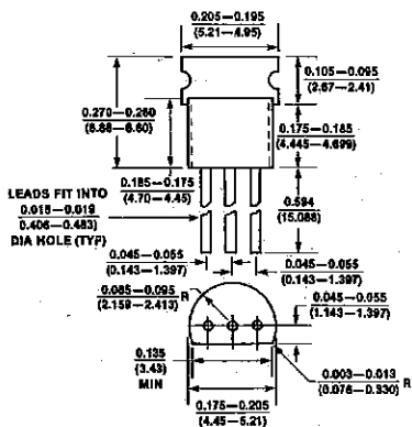
TO-237 (AR)
