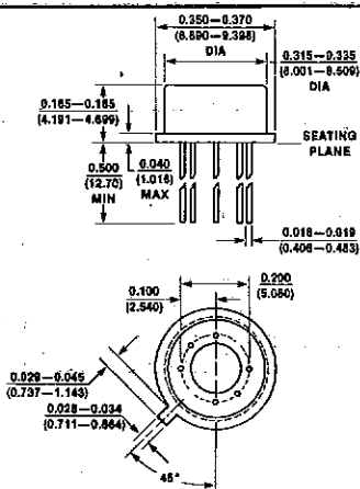
TO-78
