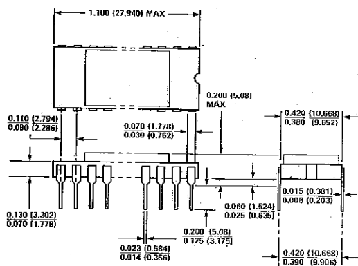
22 LEAD CERAMIC (DF)
