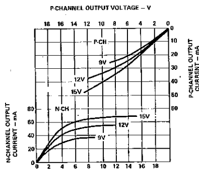
ALARM DRIVER OUTPUT CURRENT vs. OUTPUT VOLTAGE
