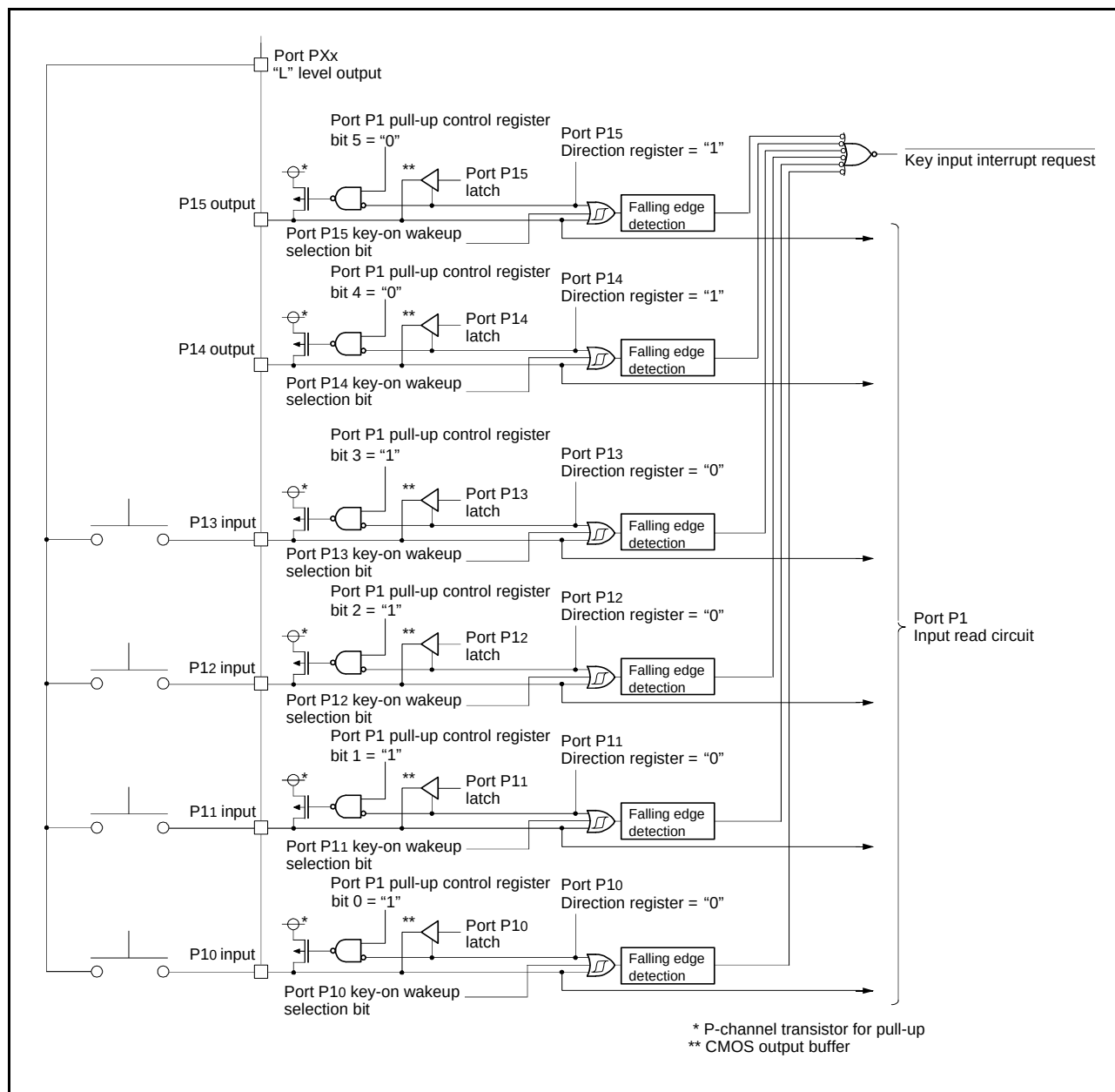
Fig 24. Connection example when using key input interrupt and port P1 block diagram
