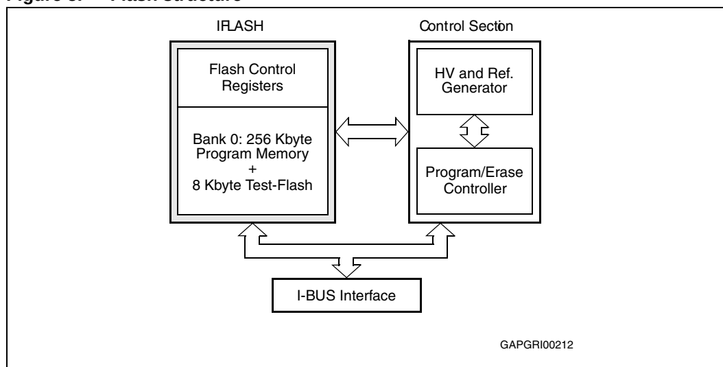
Figure 5. Flash structure
