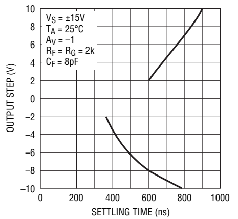
Settling Time to 150 \mu V vs Output Step
