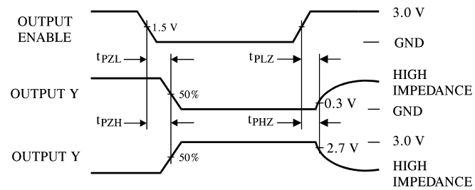
Figure 3. Switching Waveforms
